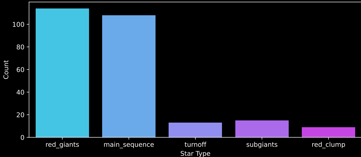
APOGEE DR17 Field: [100-18_btx] Count plot of Star Type
