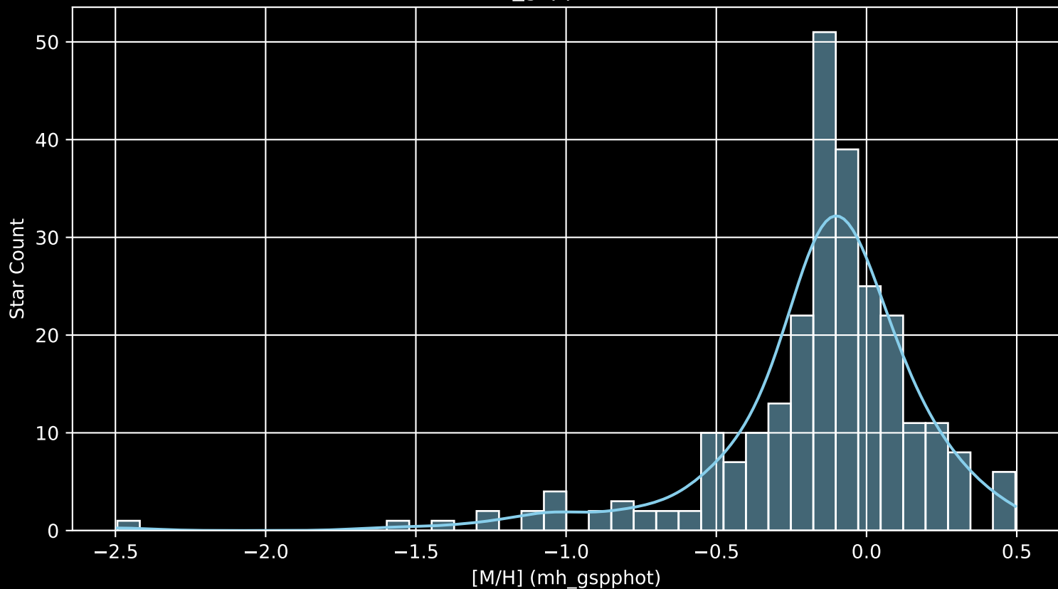
APOGEE DR17 Field: [100-18_btx [M/H] (mh_gspphot) (n= 257)
