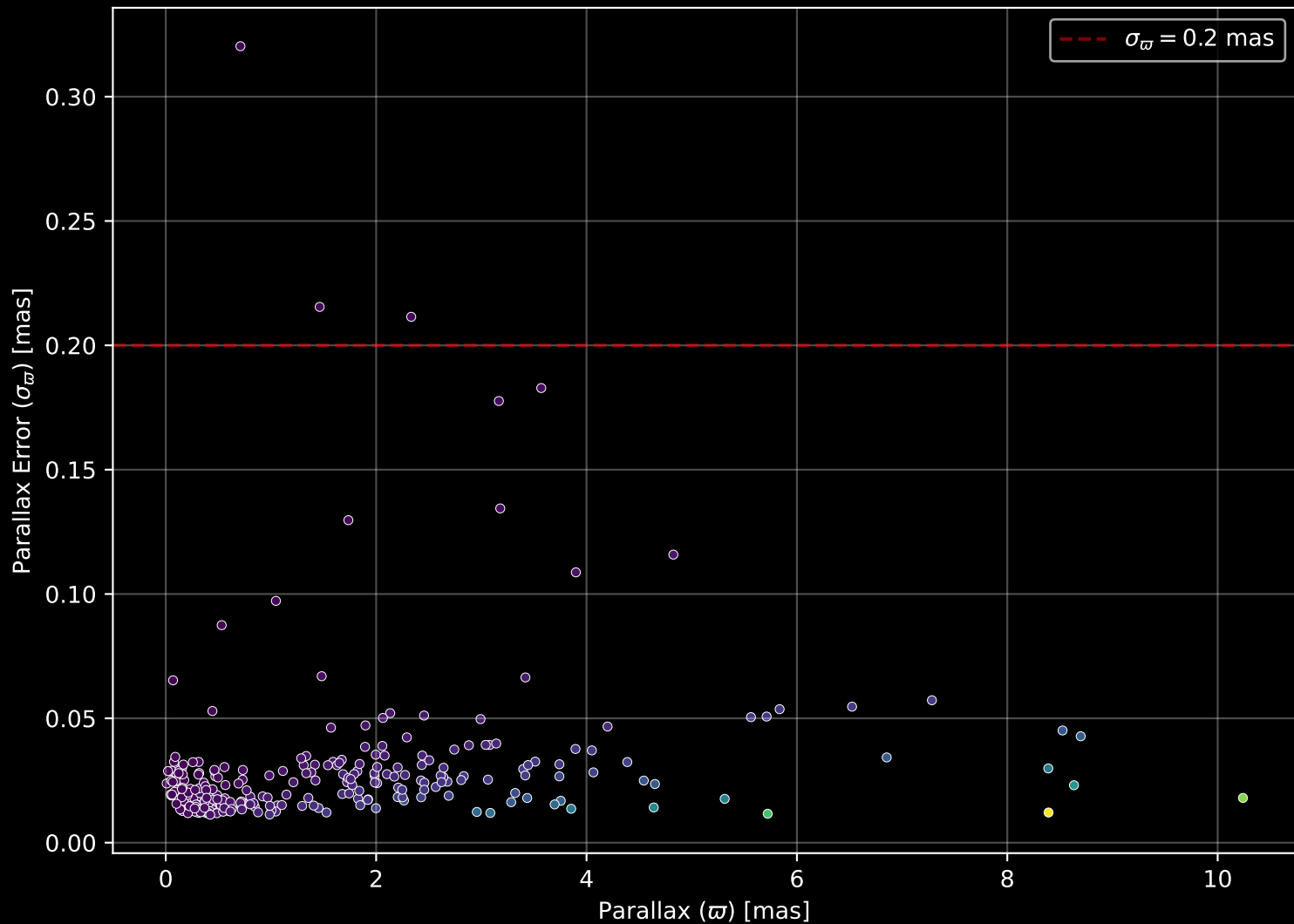
APOGEE DR17 Field: [100-18_btx] Parallax Quality (n= 259)
