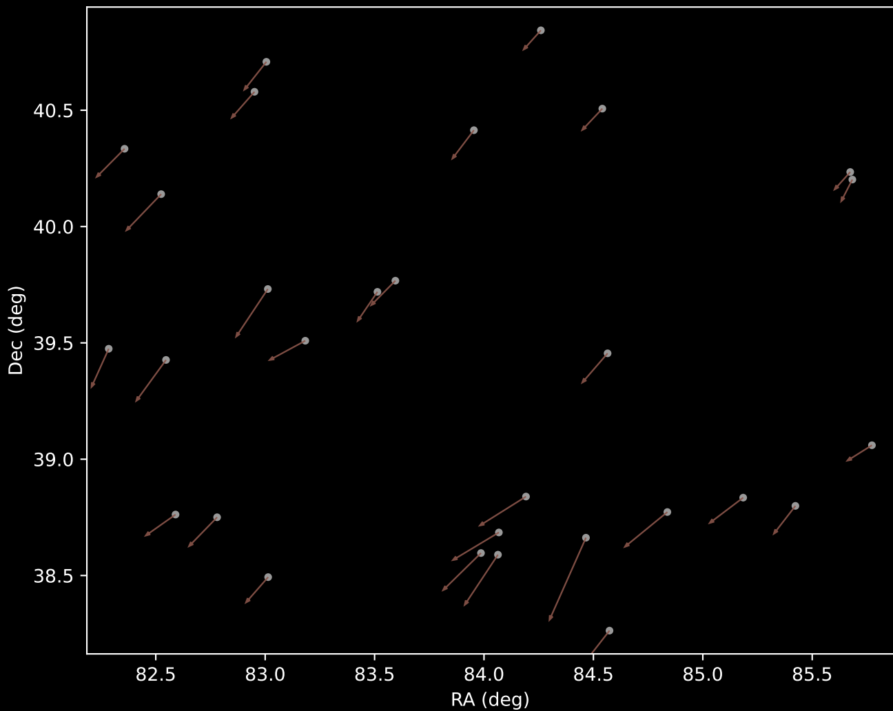
APOGEE DR17 Cluster 10 Proper Motion Vectors (n=29)
