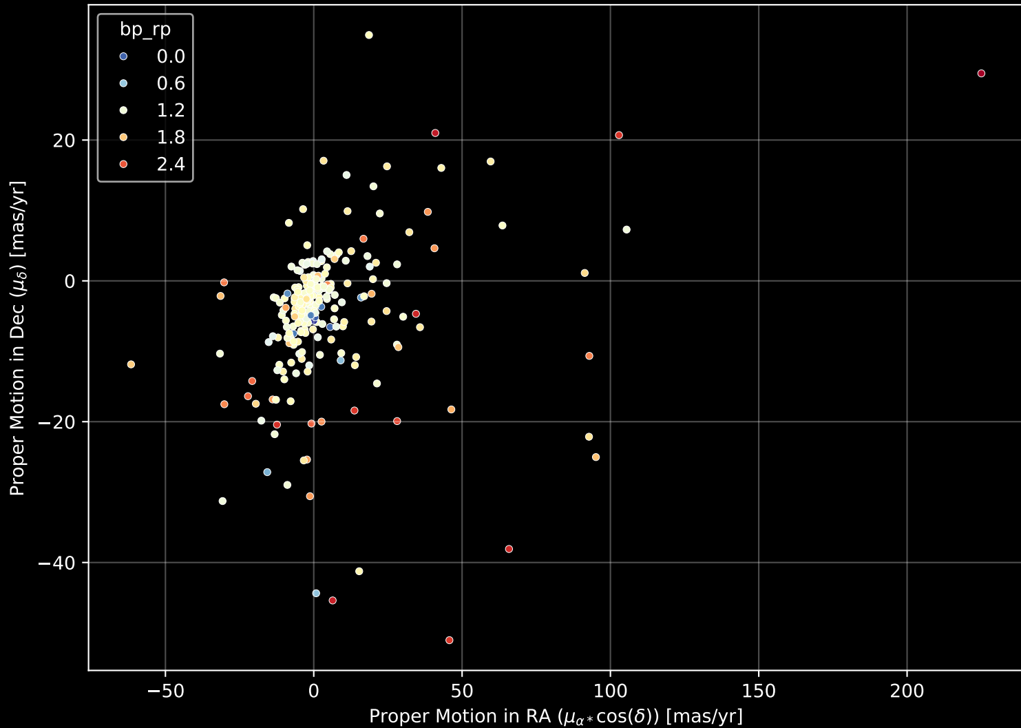
APOGEE DR17 Field: [100-18_btx] Proper Motion Diagram (n= 259)
