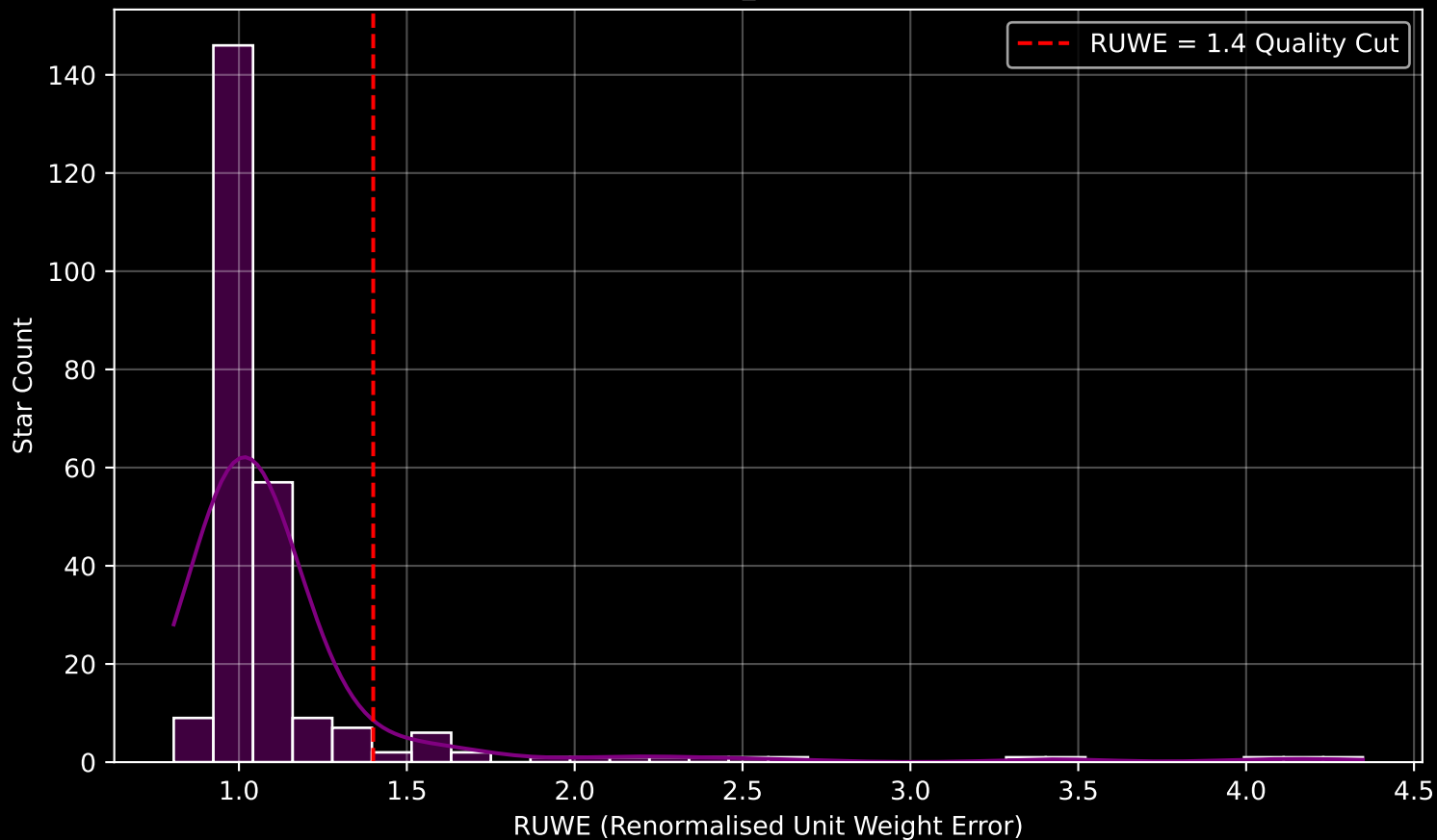
GAPOGEE DR17 Field [100-18_btx] RUWE Distribution (n= 250)
